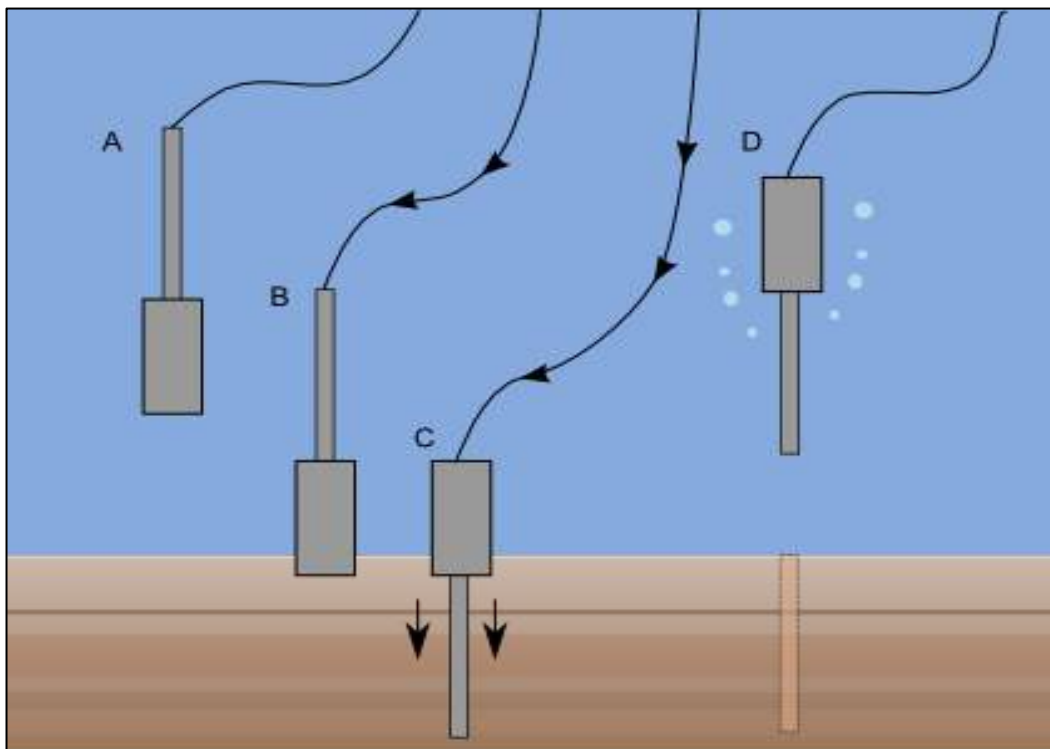
Figure 3: Mackereth corer operation. A) The device is submerged and falls under its own weight to the sediment water interface B) The system anchors itself into place as the anchor drum penetrates the sediment. C) Compressed air used to drive the coring chamber below a fixed position piston. D) Once the chamber has fully extended, air is diverted into the anchor drum, creating buoyancy that lifts the system to the surface.
