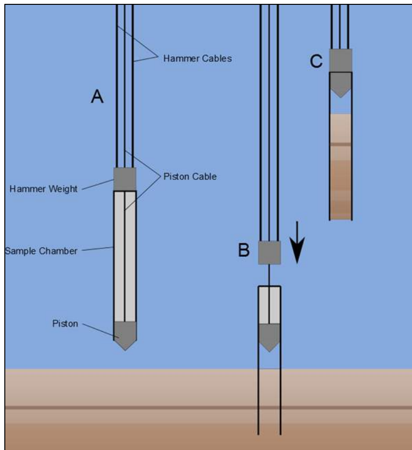
Figure 2: Wireline piston corer operation. A) The device is submerged and lowered to a short distance above the sediment water interface. B) The piston wire is secured at the surface before the sample chamber is hammered into the sediment below the fixed position piston. C) The system is raised to the surface with the sample retained in a vacuum below the piston.
