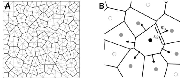
Figure 7. (A) Irregular model grid of Voronoi cells (black lines) discretised using Delaunay triangulation (grey lines) that can be used to improve model accuracy, particularly at ice body boundaries. (B) A Voronoi cell, centred on the black nodal point, Each edge of the cell has a length l_{ij} and an orientation described by the normal vector \vec{n}_{ij} . From Egholm and Nielsen (2010).
